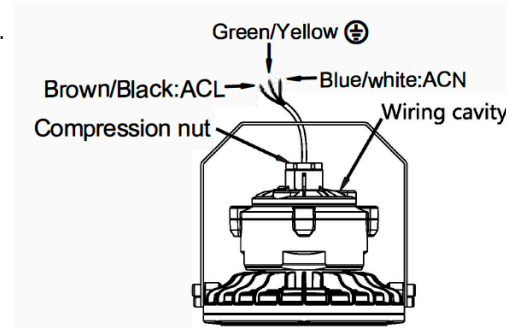
Wiring Diagram
