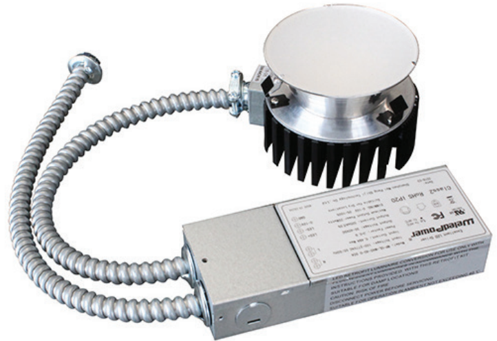
High efficiency driver and selected light engine. Fits all reflector sizes
