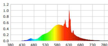
4000K Fixture Setting + Amber Optics = 2700K CCT
