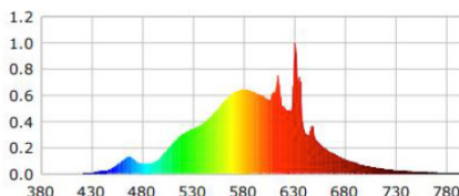
5000K Fixture Setting + Amber Optics = 3000K CCT
