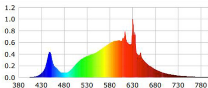
3000K Fixture Setting With Standard, Clear Optics
