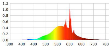
3000K Fixture Setting + Amber Optics = 2200K CCT
