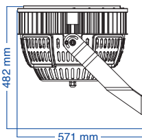
SP01B 1000W Fixture
