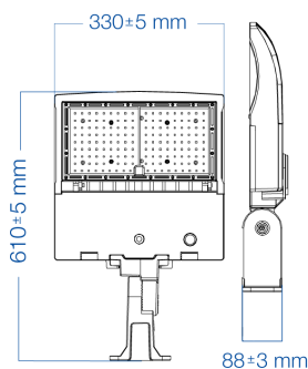
FL04B 100W-200W
