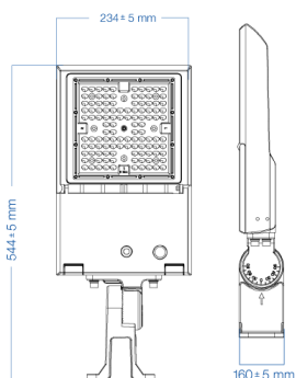
FL04B 60W-80W
