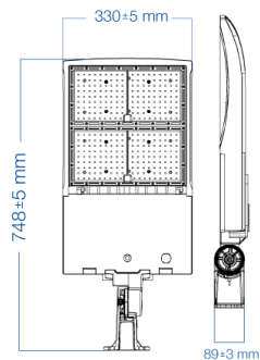
FL04B 240W-300W
